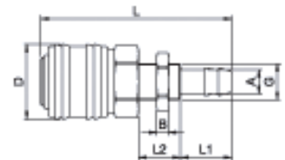
Bulkhead fitting and hose stem
