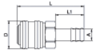
Hose stem
