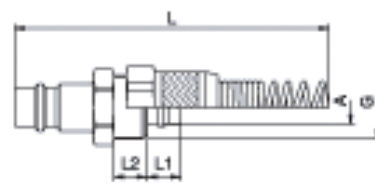
Plug for hose with swivel nut and kink protector spring
